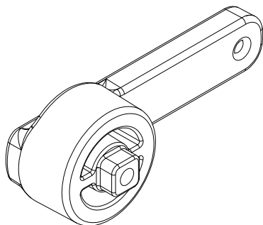
223405 KEYLOCK
