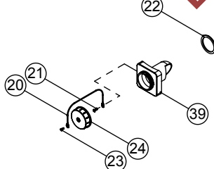
DRY USE PLASTIC FLANGE WITH BLANKING CAP
