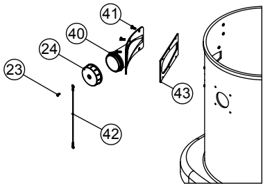
CYCLONIC INLET WITH BLANKING CAP
